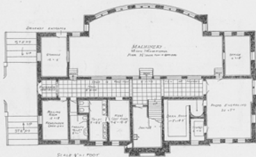
BASMENT PLAN
